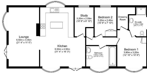
Total floor area 102.8 sq.m. (1,107 sq.ft.) approx
