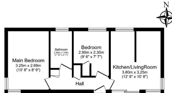
Total floor area 37.7 sq.m. (405 sq.ft.) approx
