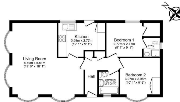
Total floor area 69.3 sq.m. (746 sq.ft.) approx
